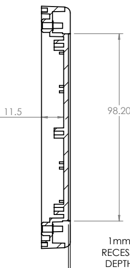
SECTION C-C
