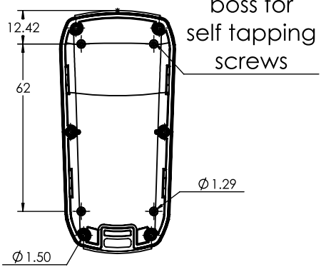
TOP COVER
