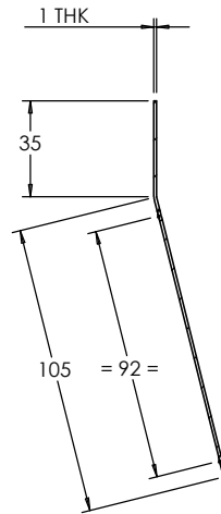
SECTION B-B
