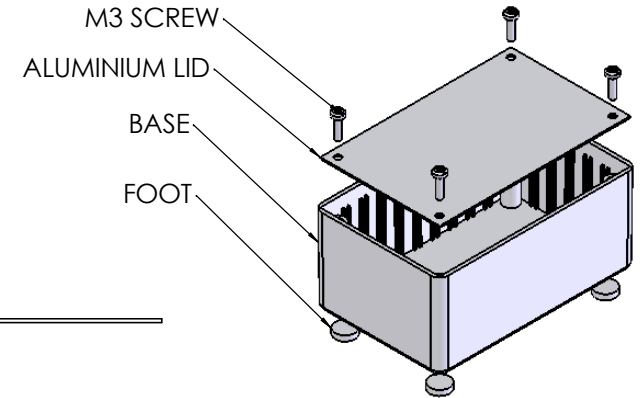
ISO VIEW 1:3
