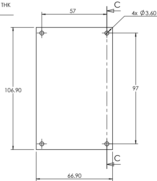
SECTION C-C
